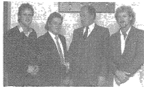
The Chairman of the Executive Mr. Jim Hawkins congratulates Scott Cowley of Old Trinity, winner of the D Section Best & Fairest. Looking on are T. Lawley of West Brunswick, third and A. Turchett of North Brunswick, second.
